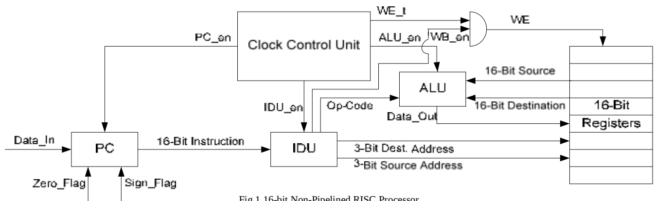
Fig.1 16-bit Non-Pipelined RISC Processor
