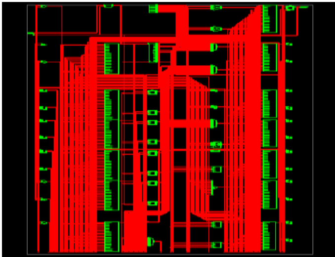
Fig. 4 RTL Schematic of RISC Processor
