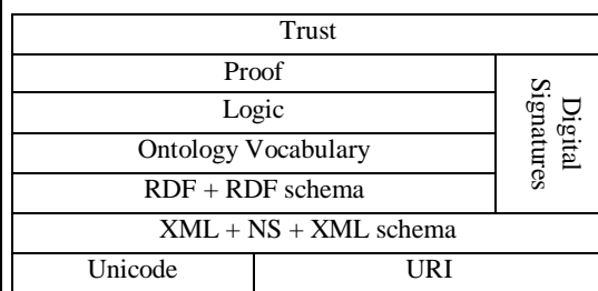
FIGURE 2. ARCHITECTURE OF THE SEMANTIC WEB
